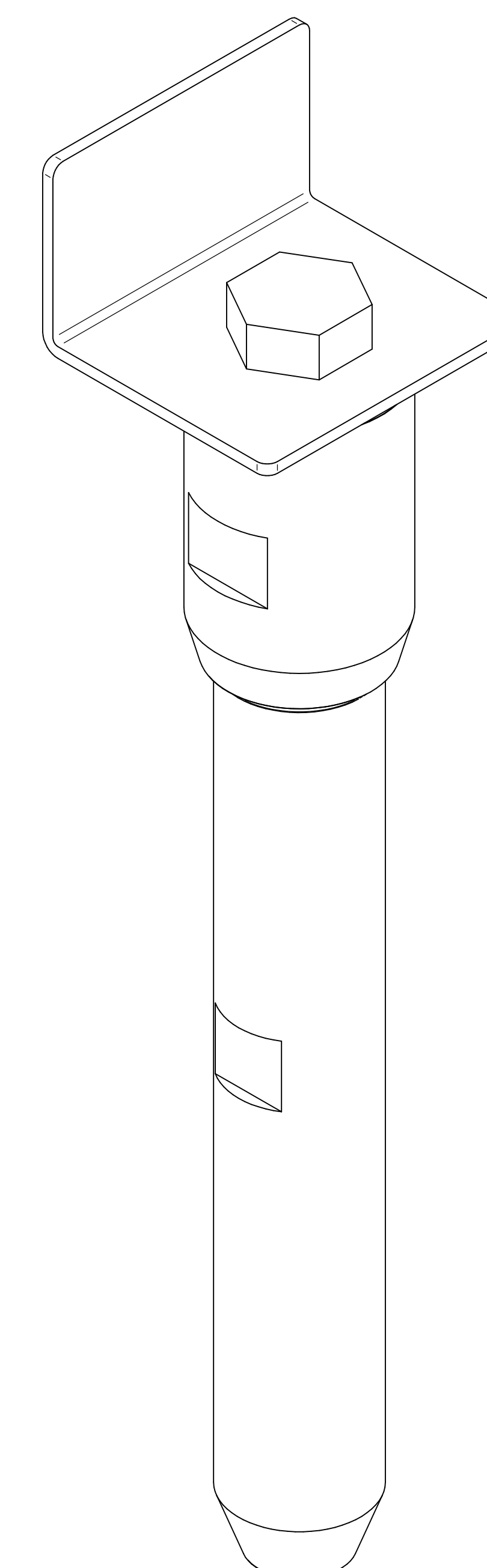
ISOMETRIC VIEW
