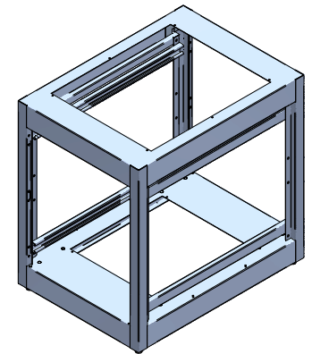
ISOMETRIC
