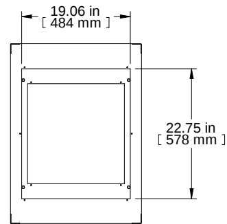
TOP VIEW TOP OPENING
