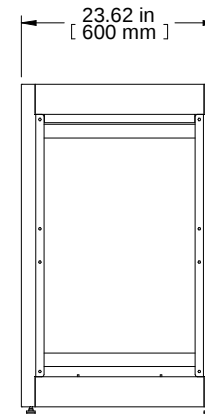
R.S. VIEW
