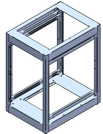
ISOMETRIC
