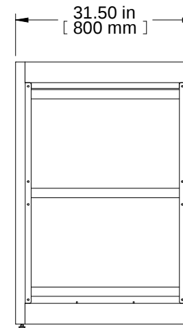
R.S. VIEW
