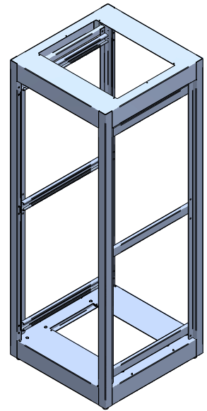
ISOMETRIC
