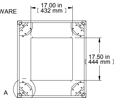
BOTTOM VIEW BOTTOM OPENING
