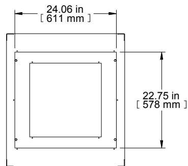
TOP VIEW TOP OPENING
