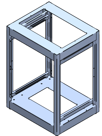
ISOMETRIC
