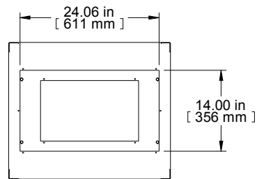
TOP VIEW TOP OPENING
