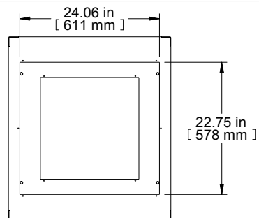
TOP VIEW TOP OPENING
