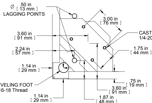
DETAIL A 4X SCALE 5:1
