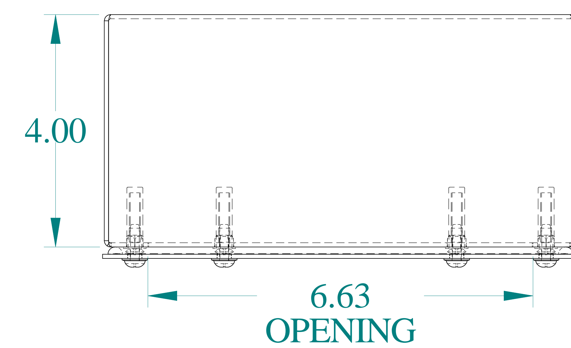
TOP VIEW
