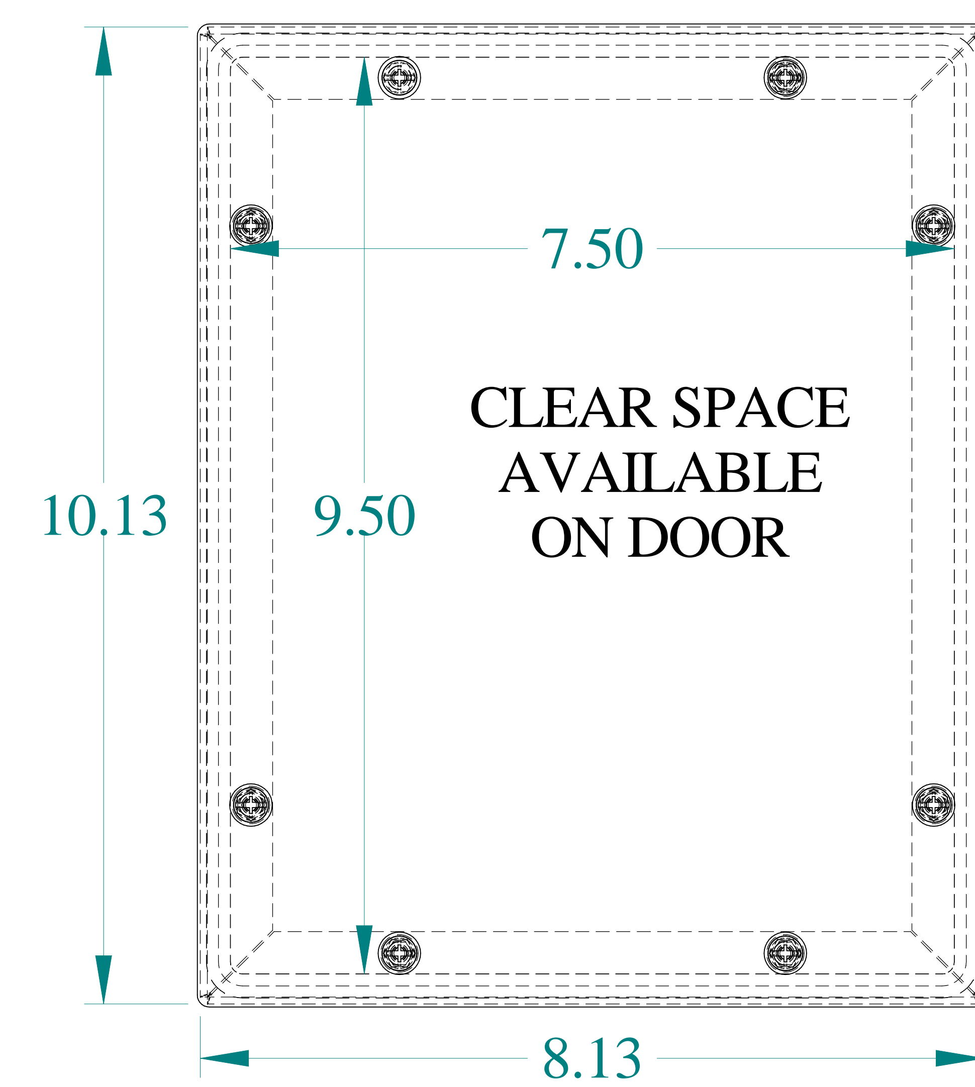
FRONT VIEW
