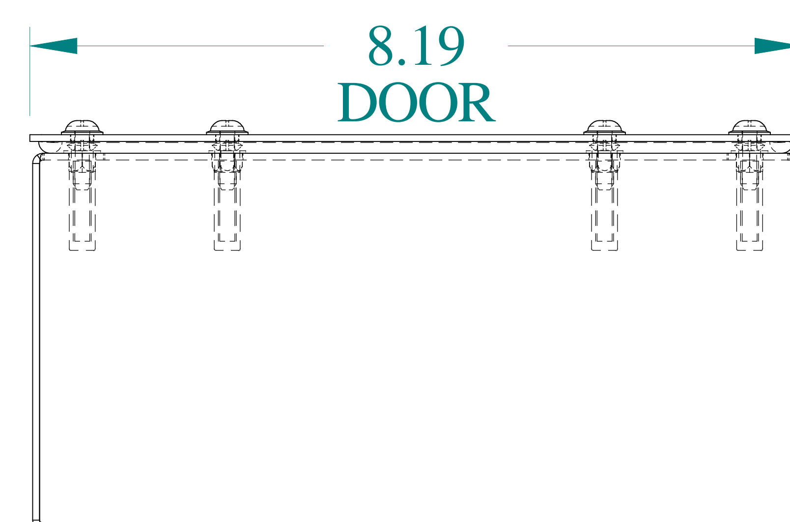
BOTTOM VIEW
