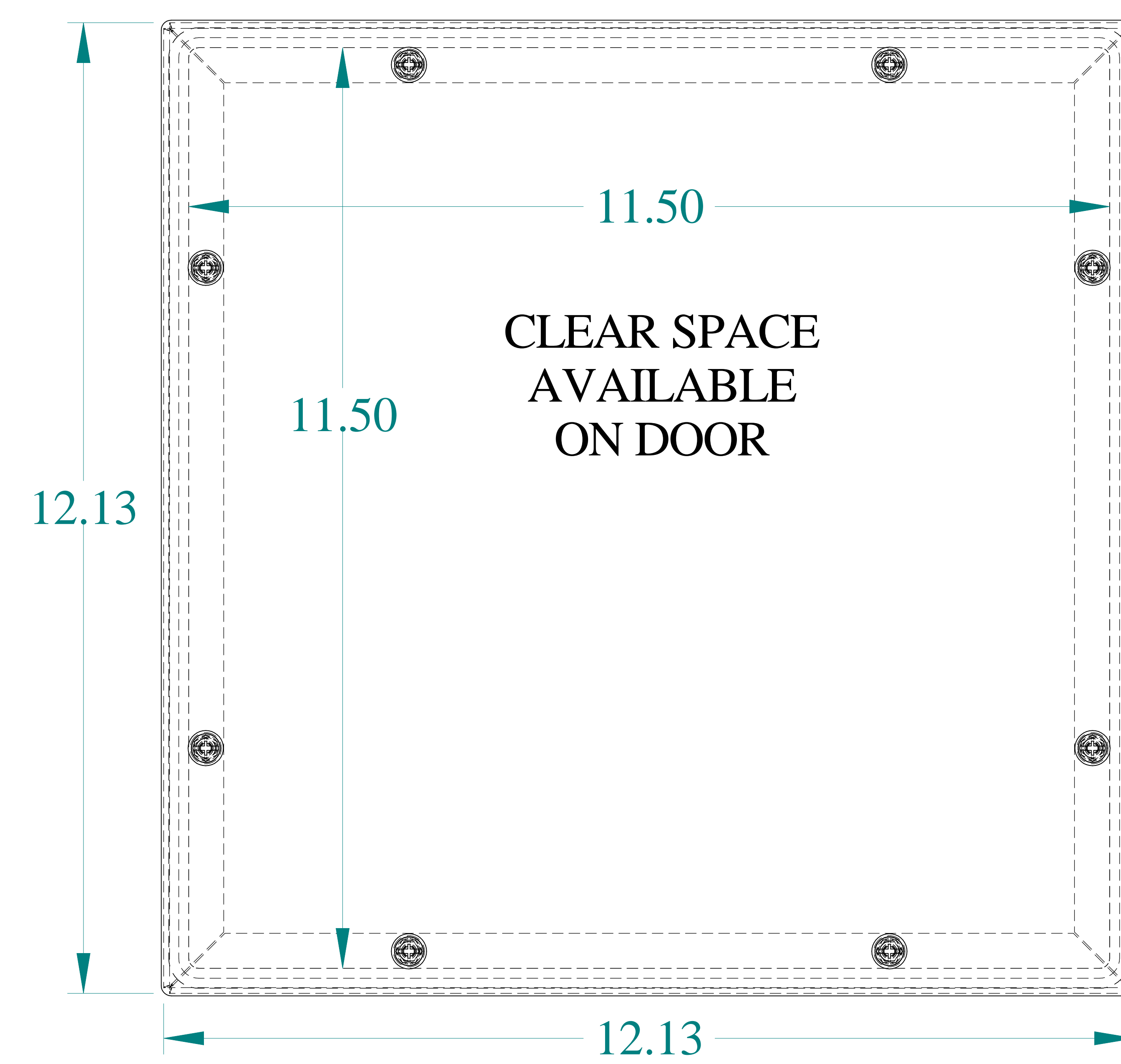
FRONT VIEW
