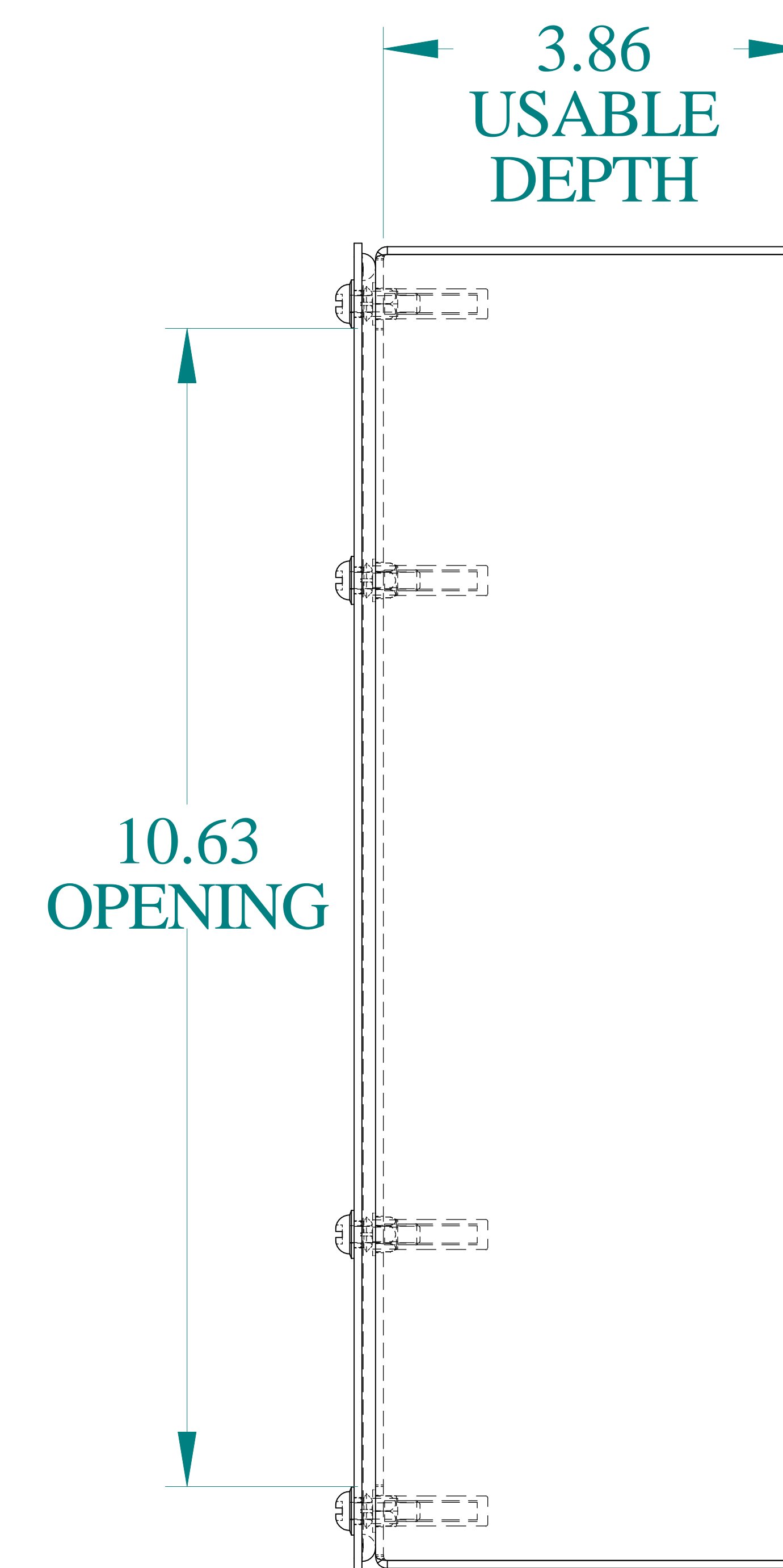
SIDE VIEW
