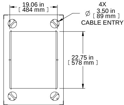
TOP VIEW TOP OPENING
