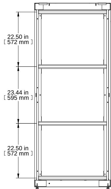
SECTION B-B
