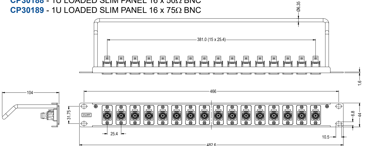
CP30188 - 1U LOADED SLIM PANEL 16 x 50 \Omega BNC
