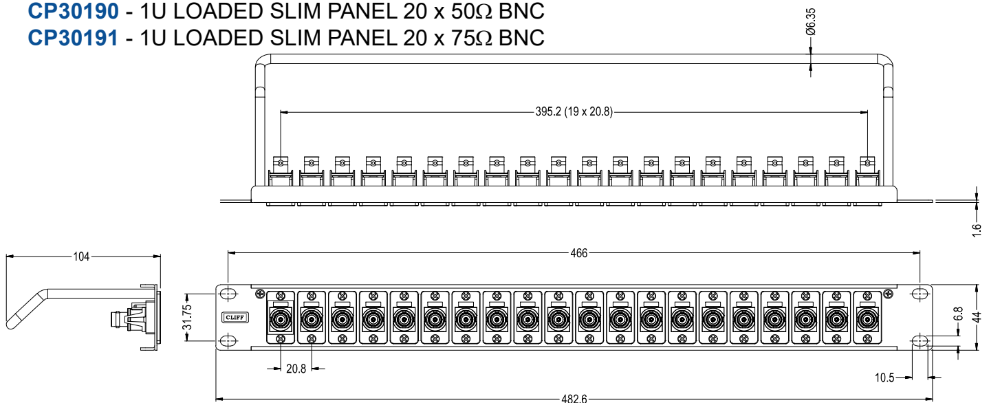
CP30190 - 1U LOADED SLIM PANEL 20 x 50 \Omega BNC
