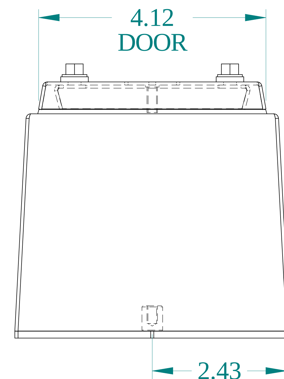
BOTTOM VIEW
