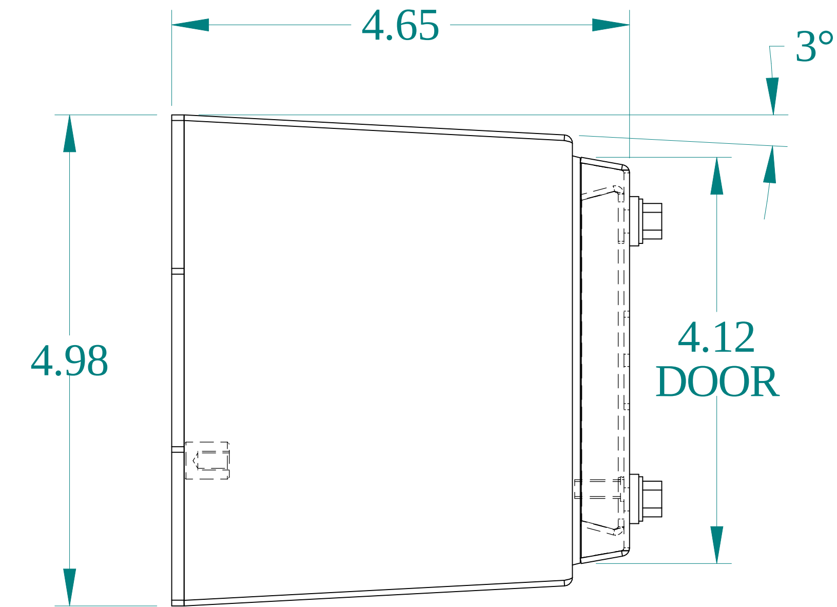
SIDE VIEW
