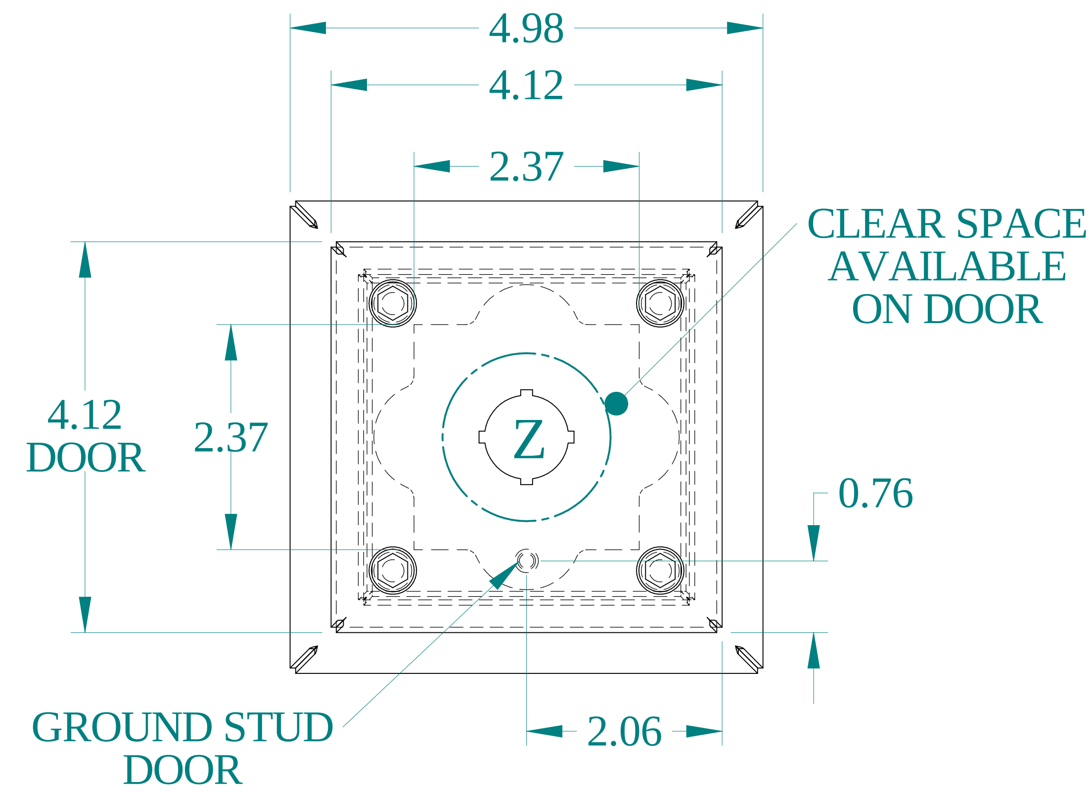
TOP VIEW
