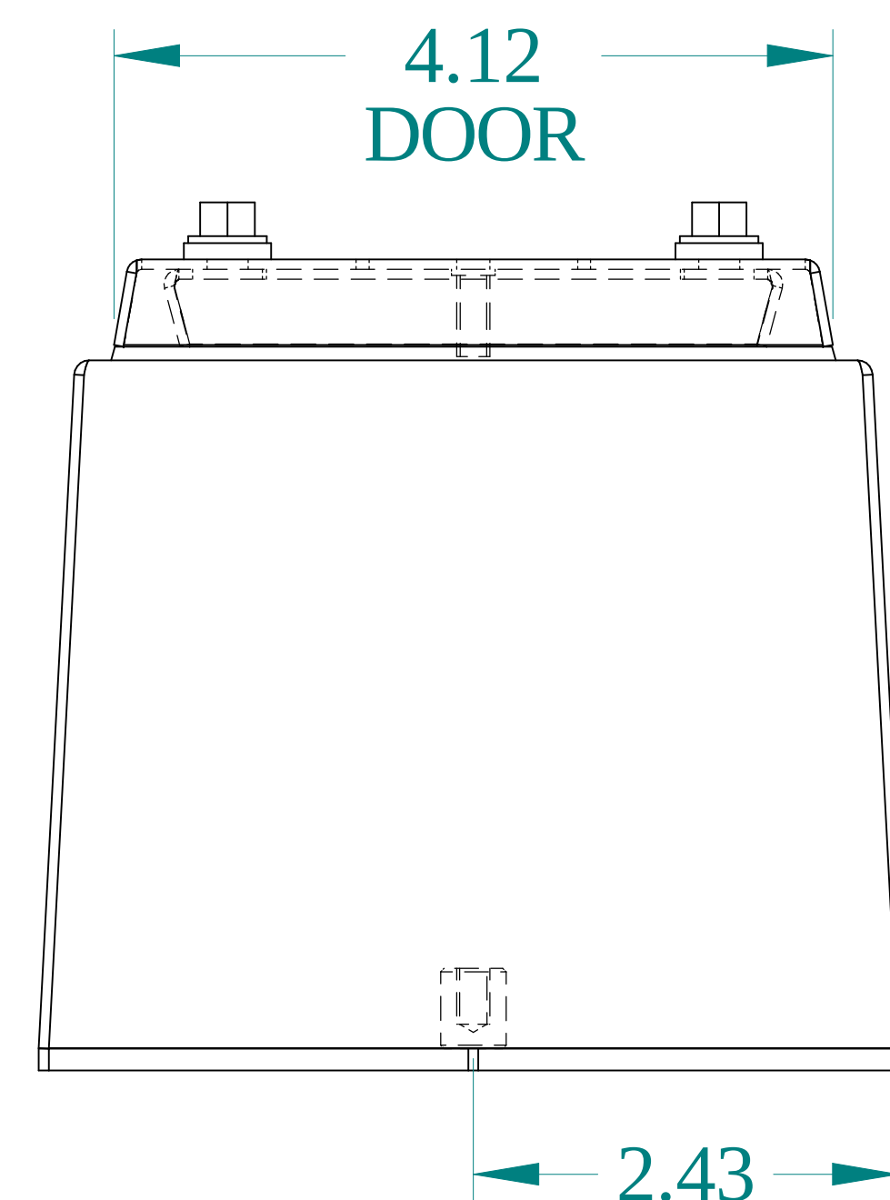
BOTTOM VIEW
