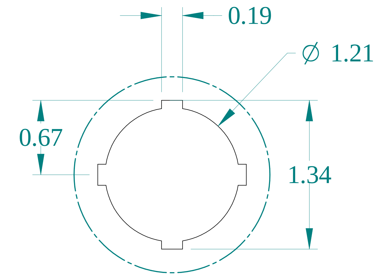
DETAIL Z
