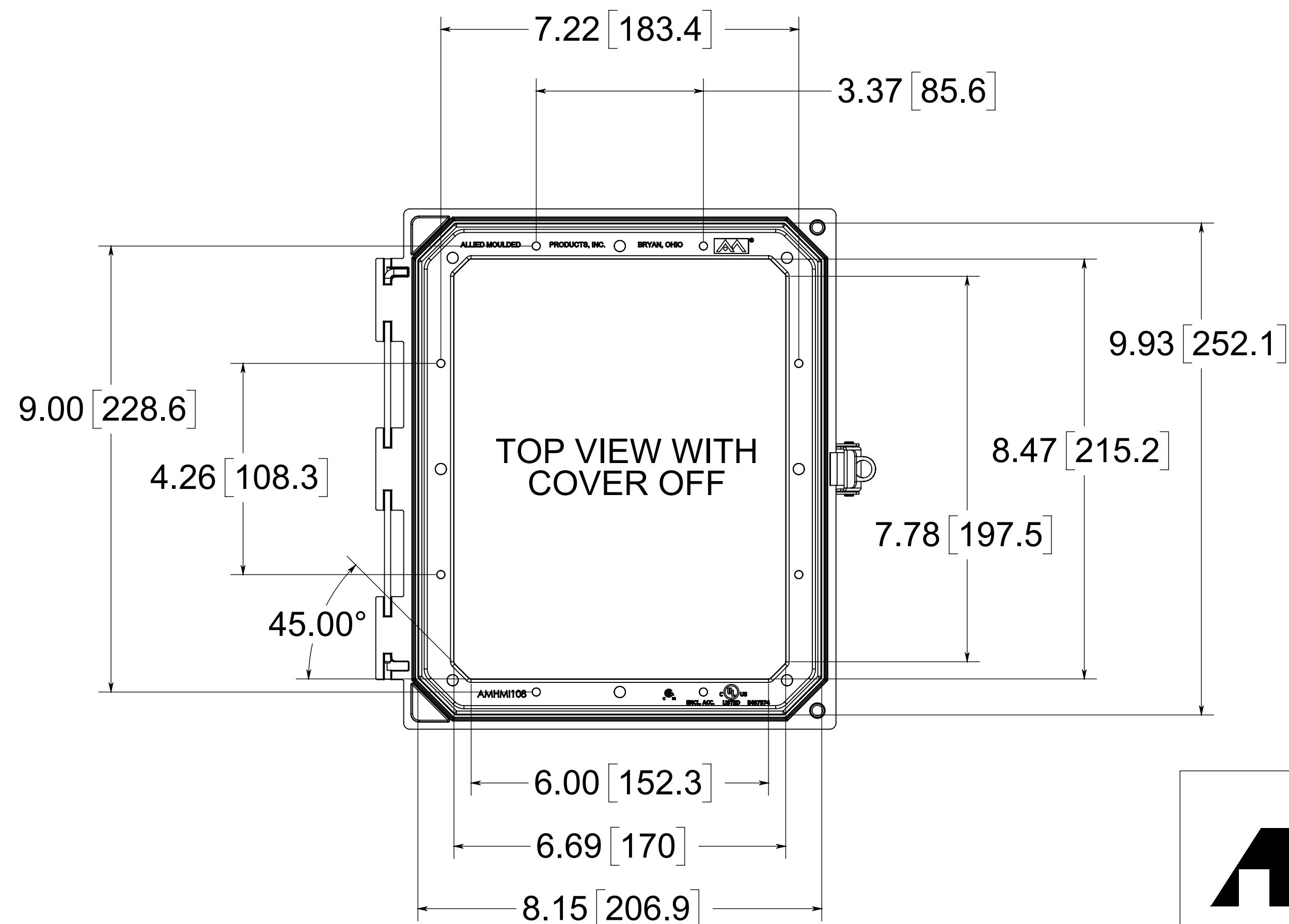
MOUNTING HOLE PATTERN HMI108
