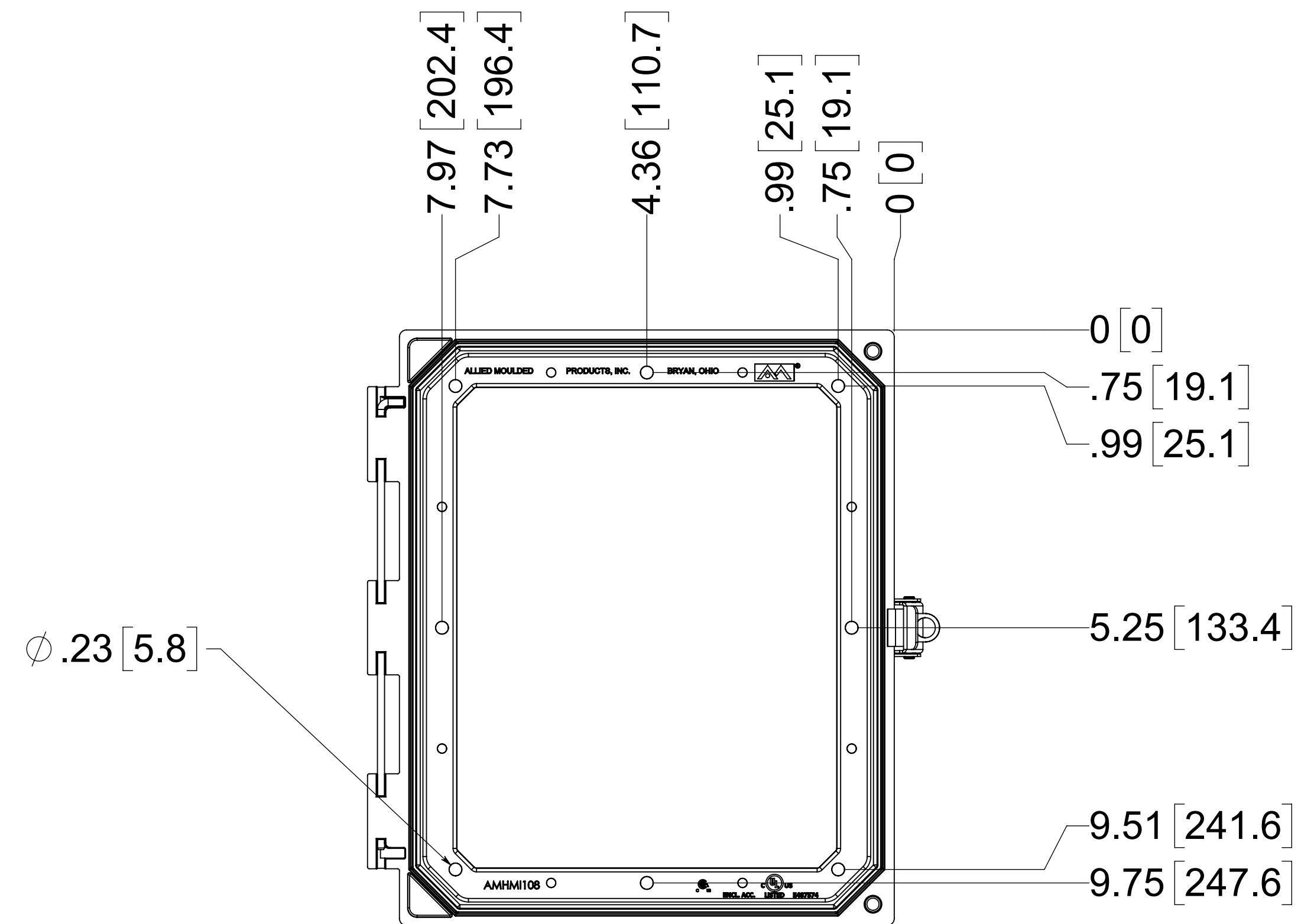
MOUNTING HOLE PATTERN HMI108
