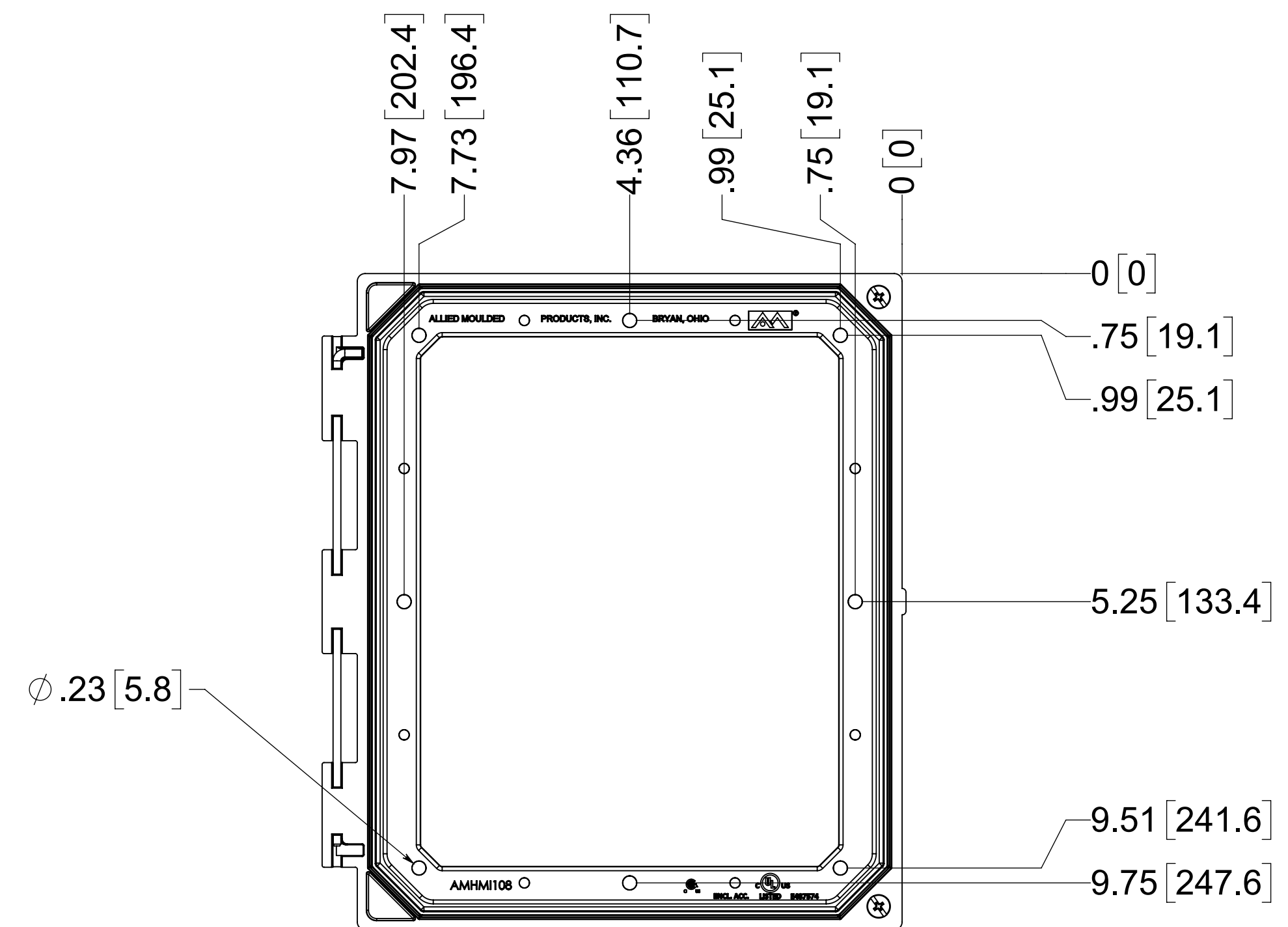
MOUNTING HOLE PATTERN HMI108
