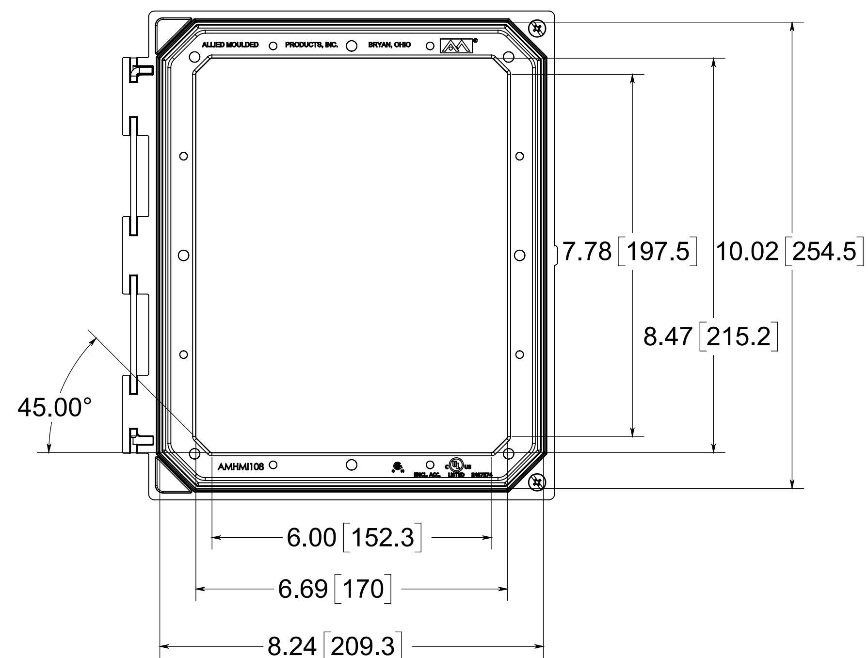
TOP VIEW WITH COVER OFF
