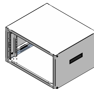
ISOMETRIC
