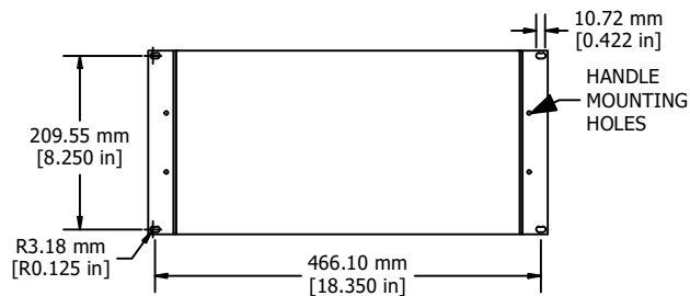
ASSEMBLY - FRONT VIEW
