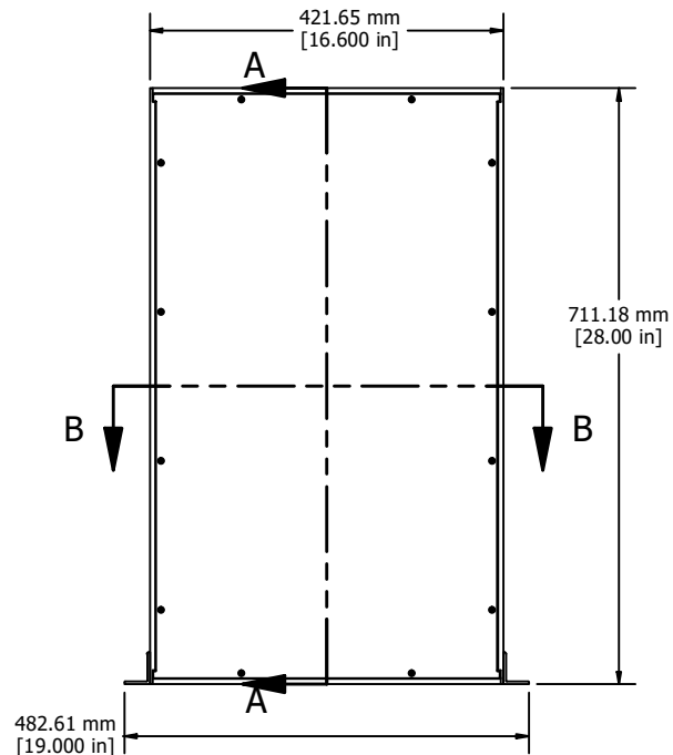
ASSEMBLY - TOP VIEW
