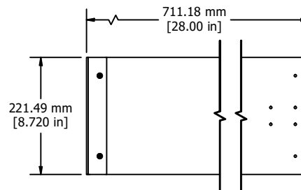
ASSEMBLY - SIDE VIEW
