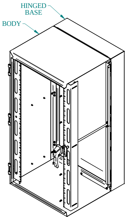
ISOMETRIC VIEW (FRONT DOOR & RH SIDE REMOVED)
