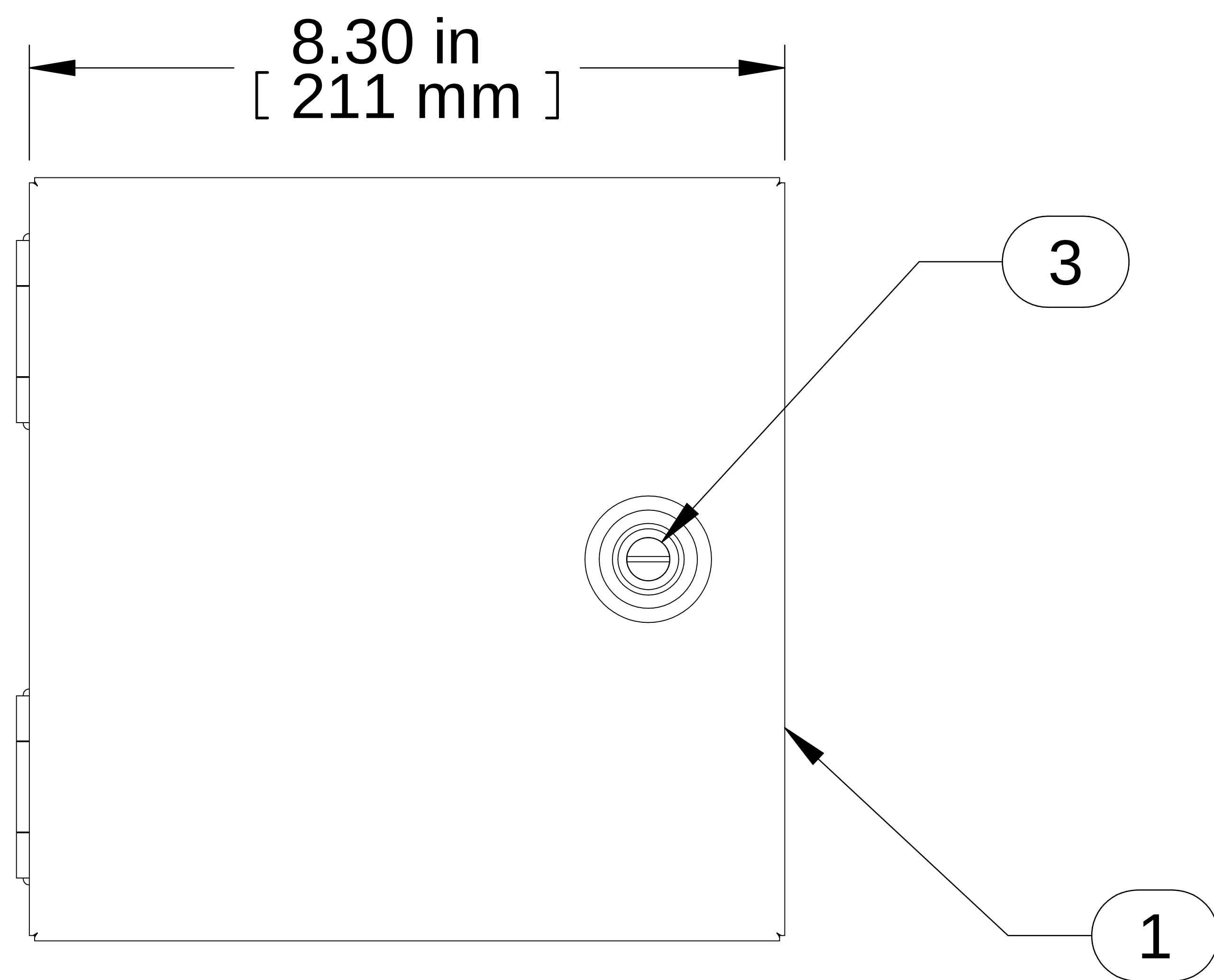
TOP VIEW
