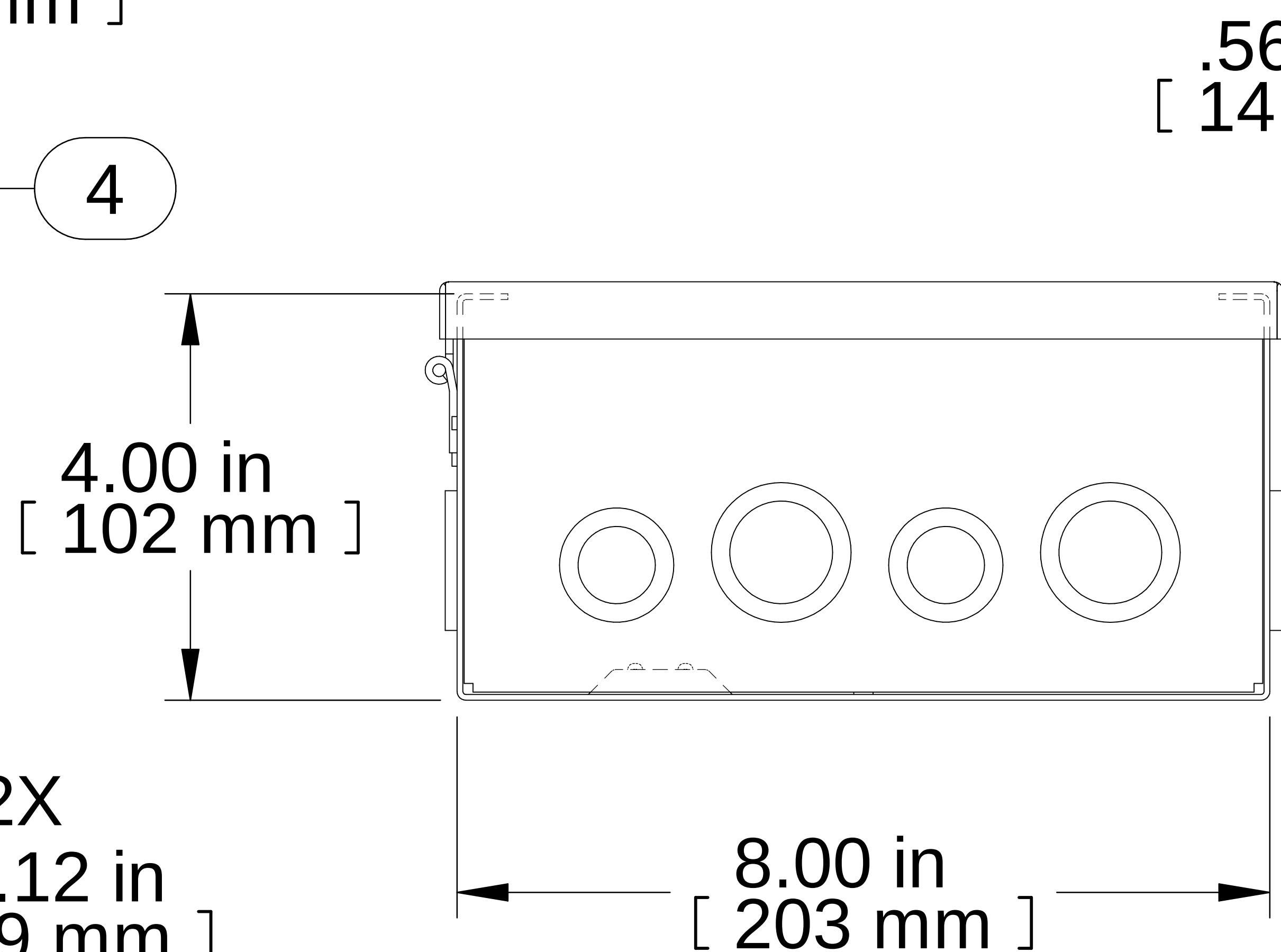
FRONT VIEW
