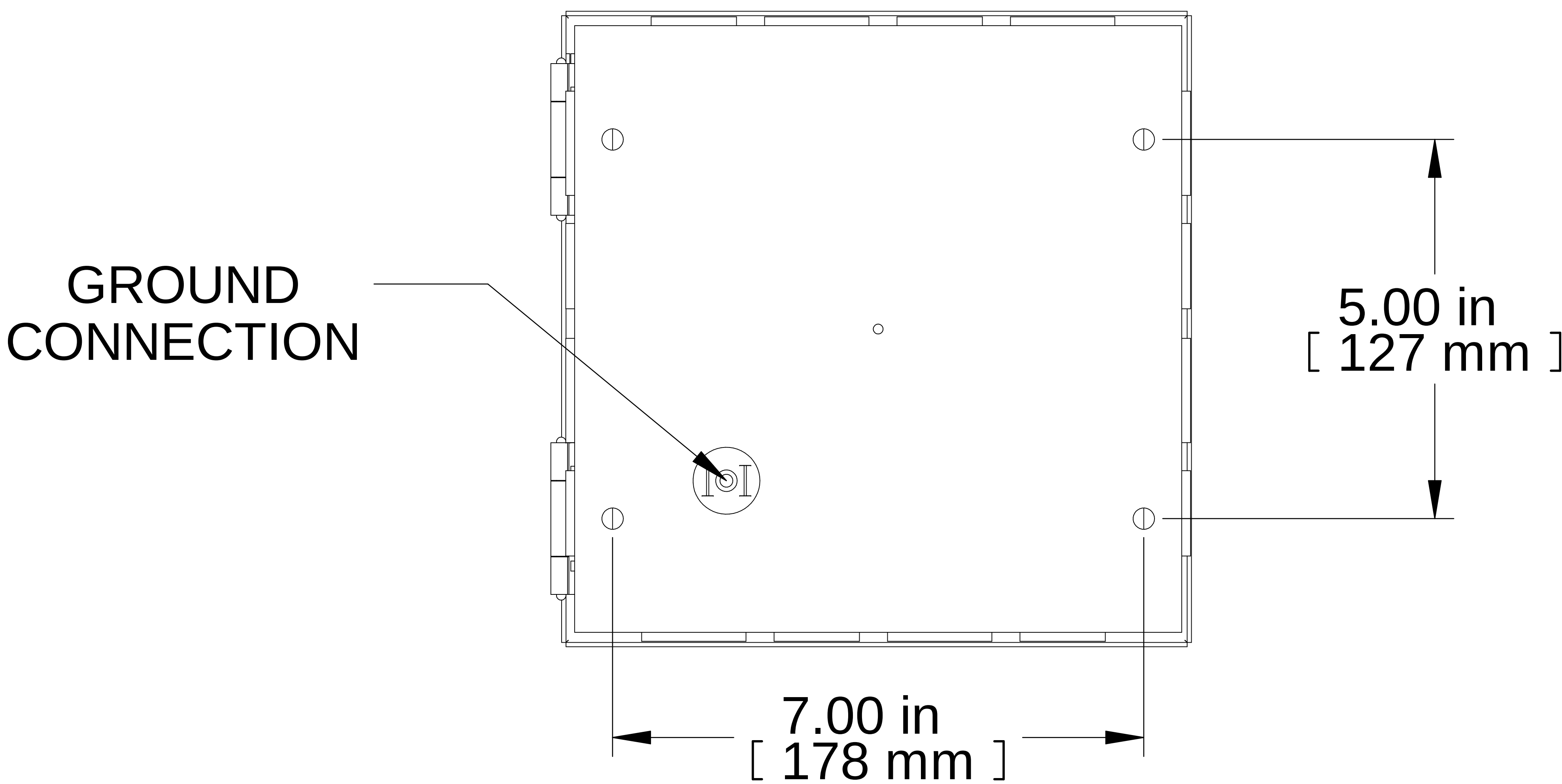
BOTTOM VIEW
