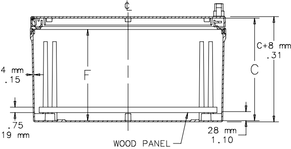
SECTION X-X
