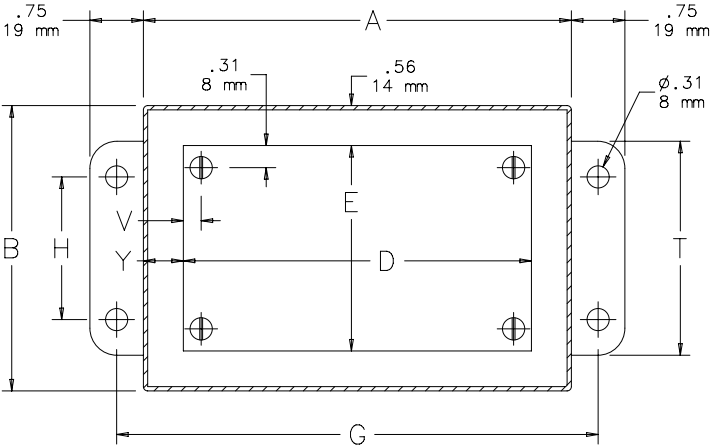
SECTION Y-Y
