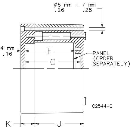
SECTION C-C
