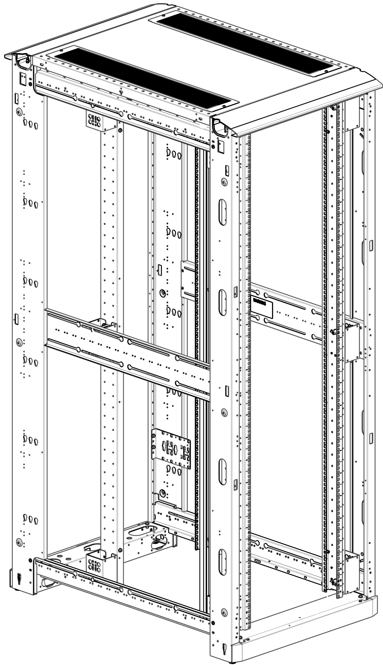
FRONT ISO
