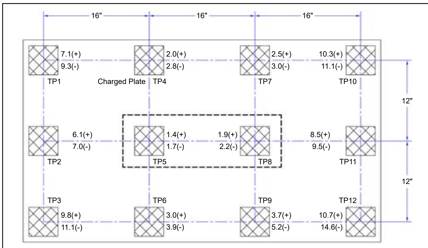
Figure 15. 60640, 60467 Neutralization (Discharge) Times at 120VAC, 60Hz input
