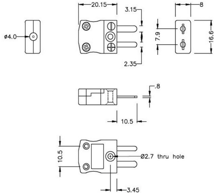
Miniature in-line Plug (dimensions in mm)
