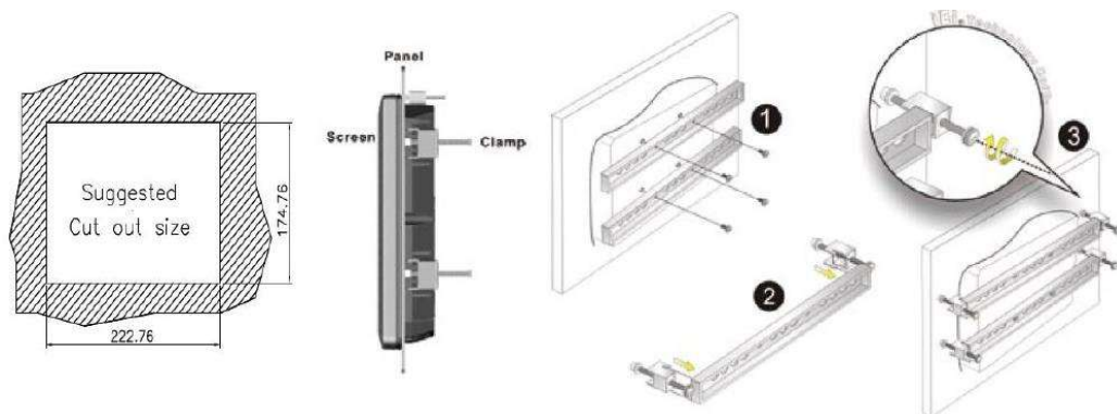
Figures 2. Mounting Drawing
