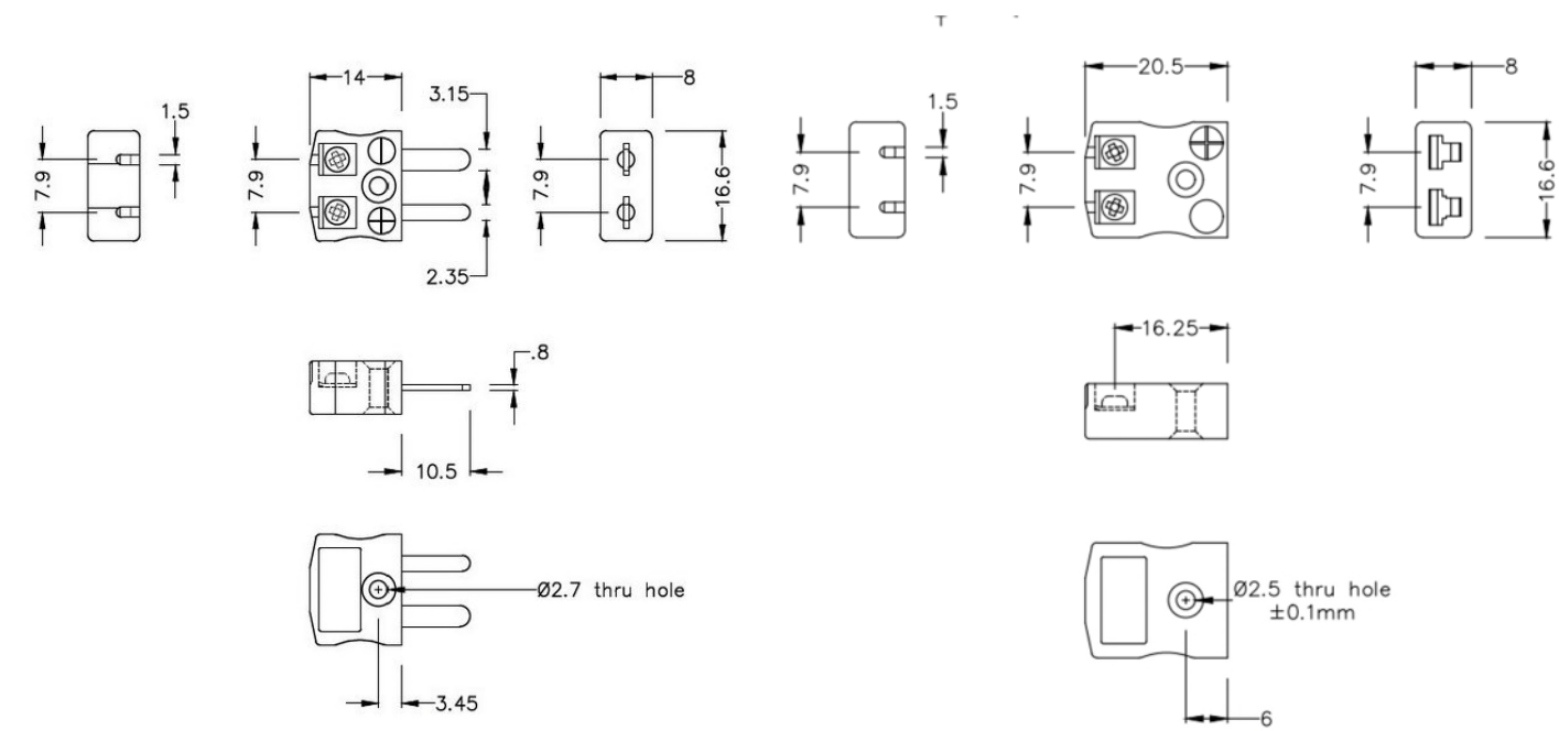
Miniature in-line Plug - Quick Wire (dimensions in mm)
