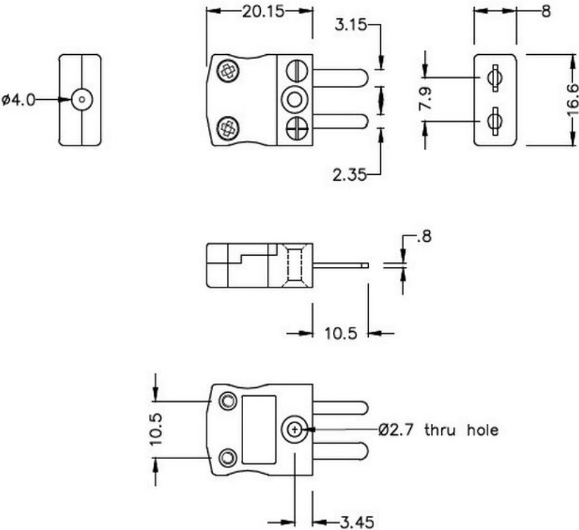
Miniature in-line Plug (dimensions in mm)
