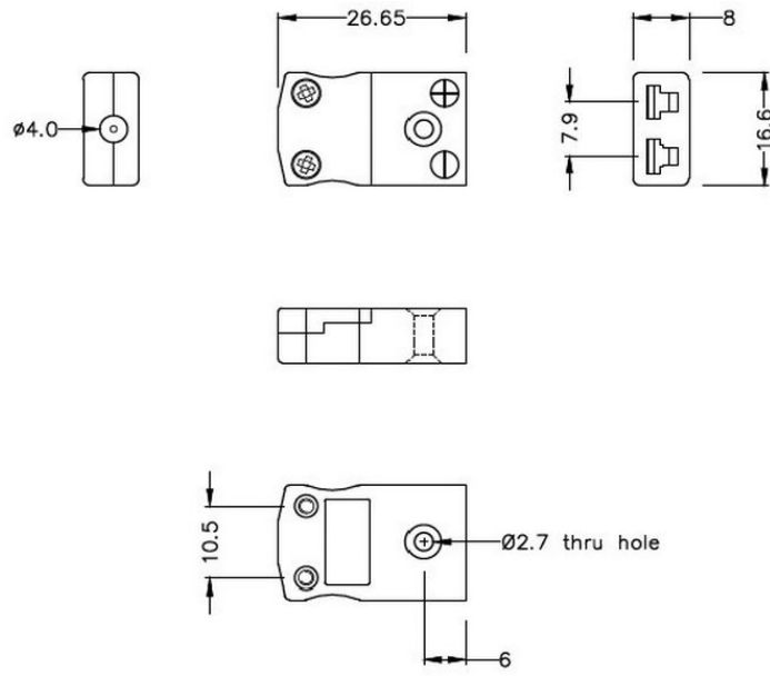
Miniature in-line Socket (dimensions in mm)
