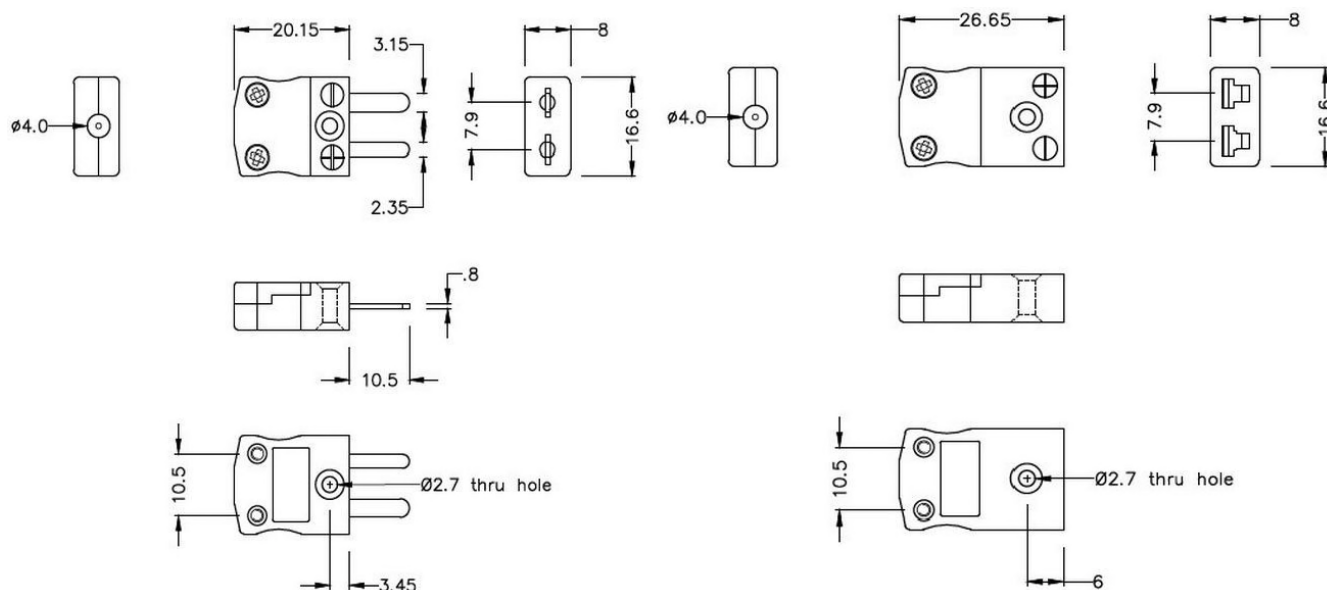
Miniature in-line Plug (dimensions in mm)
