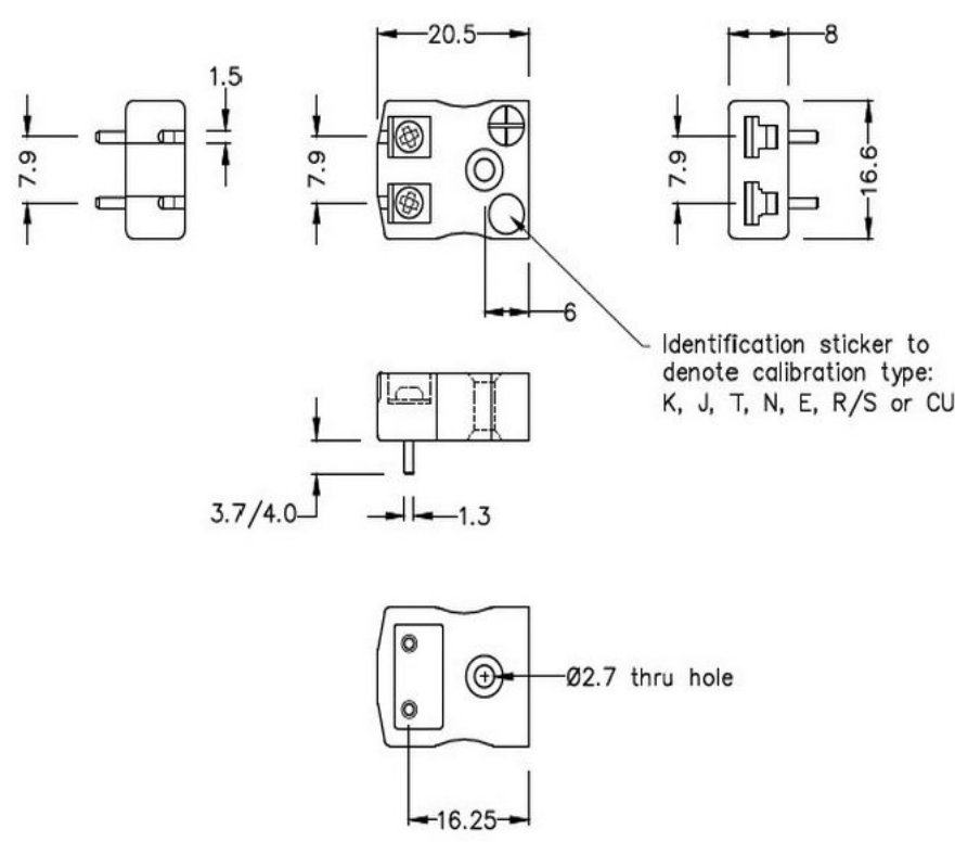
Miniature PCB Socket (dimensions in mm)
