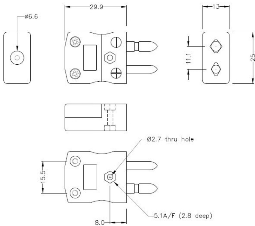
Standard in-line Plug (dimensions in mm)
