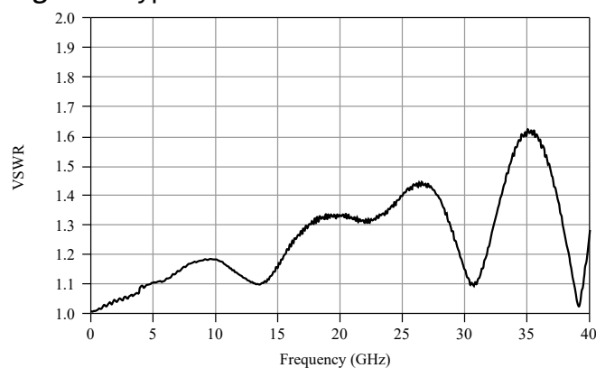
Figure 3. Typical VSWR
