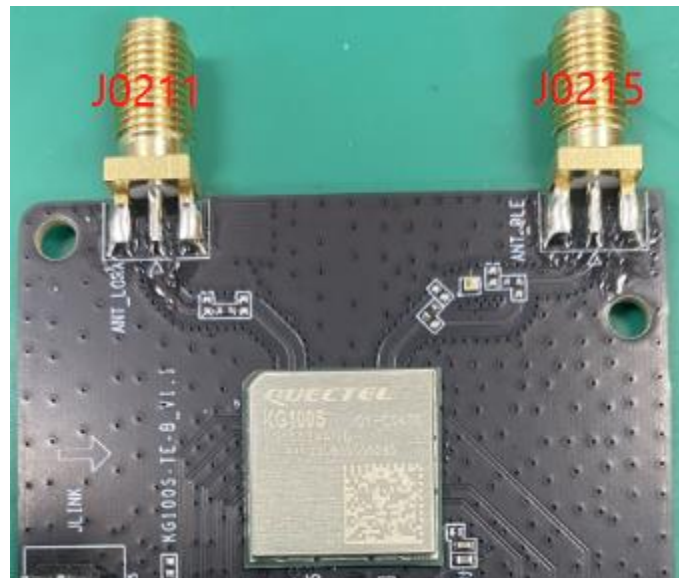
Figure 12: RF Connectors
