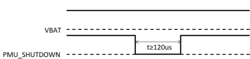
Figure 5.3 Power Sequence Diagram – Power Up
