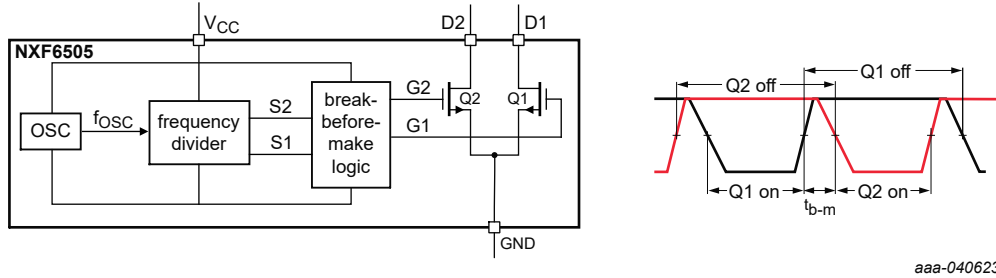
Fig. 79. Block diagram and output timing with break-before-make action
