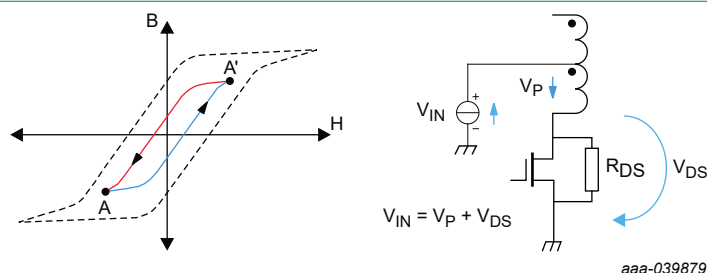
Fig. 6. Core magnetization and self-regulation through positive temperature coefficient of R_{DS(on)}
