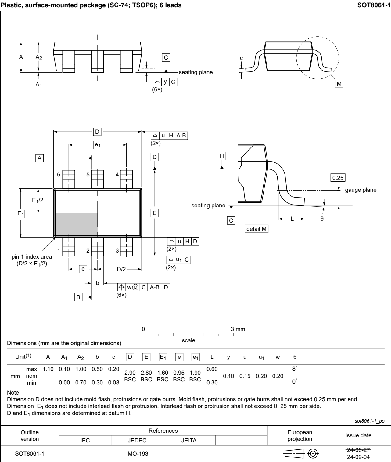
Fig. 84. Package outline SOT8061-1 (SC-74; TSOP6)
