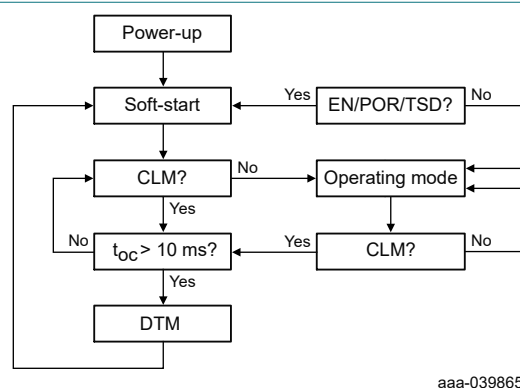
Fig. 7. State machine flow for the overcurrent protection mode
