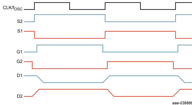
Fig. 80. Output signal waveforms
