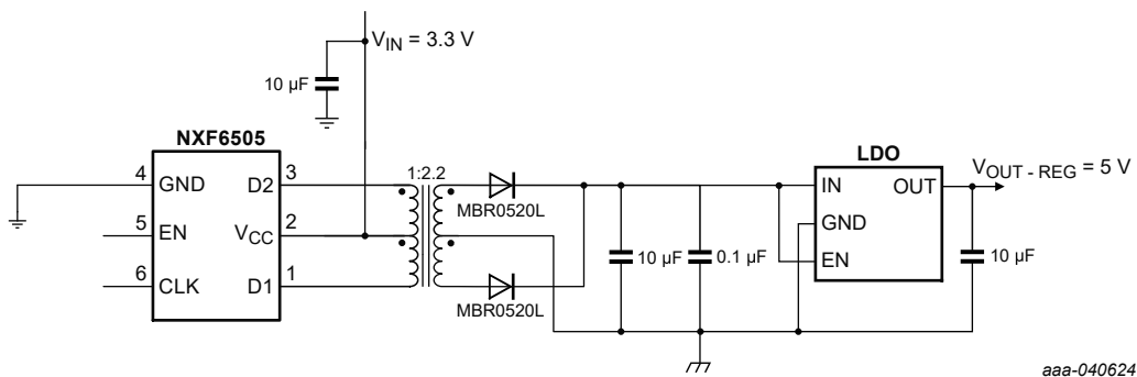
Fig. 81. NXF6505-Q100 typical application schematic
