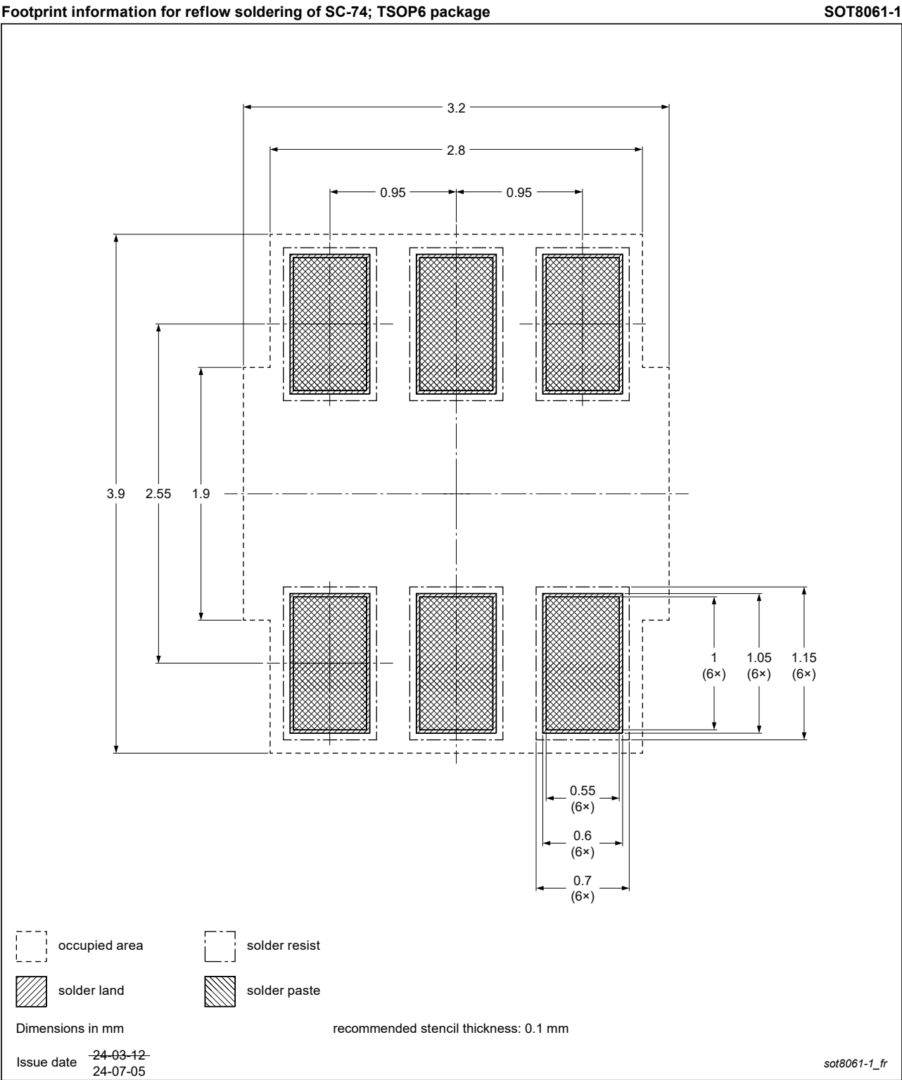
Fig. 85. Reflow soldering footprint SOT8061-1 (SC-74; TSOP6)
