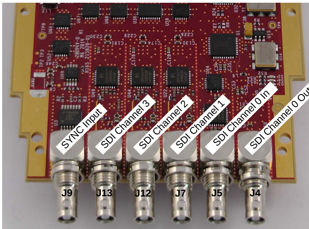
Figure 8-1 TB-FMCH-12GSDI Front Edge HDBNC Coaxial Connectors
