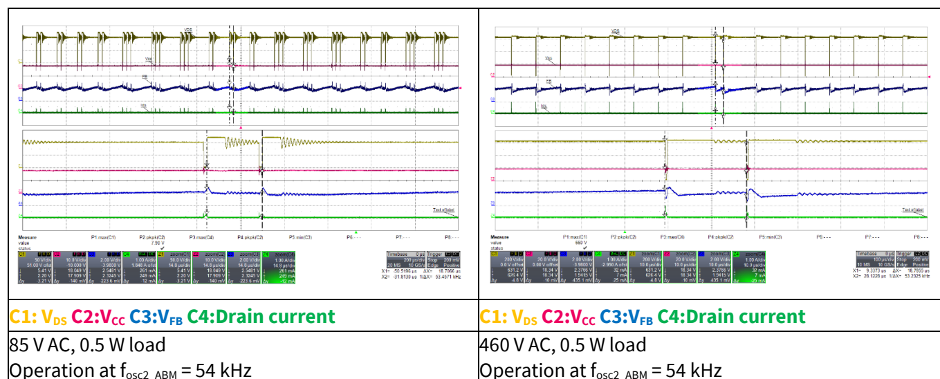
Figure 17 ABM operation
