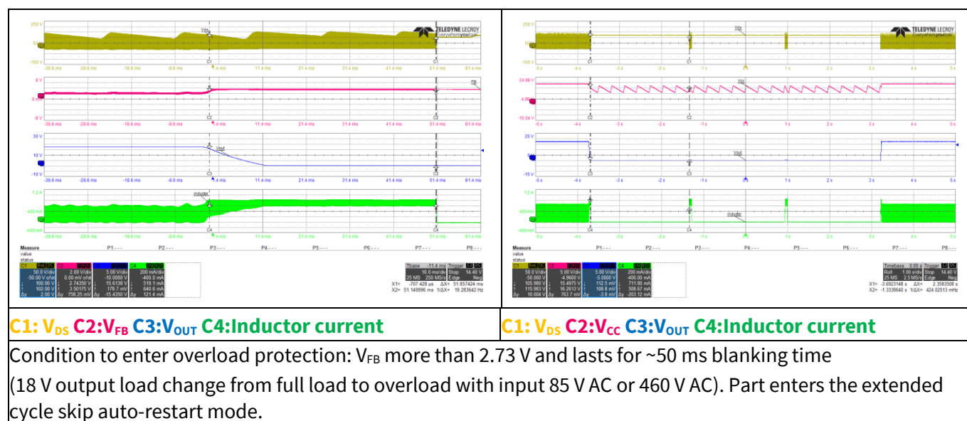
Figure 18 Overload protection
