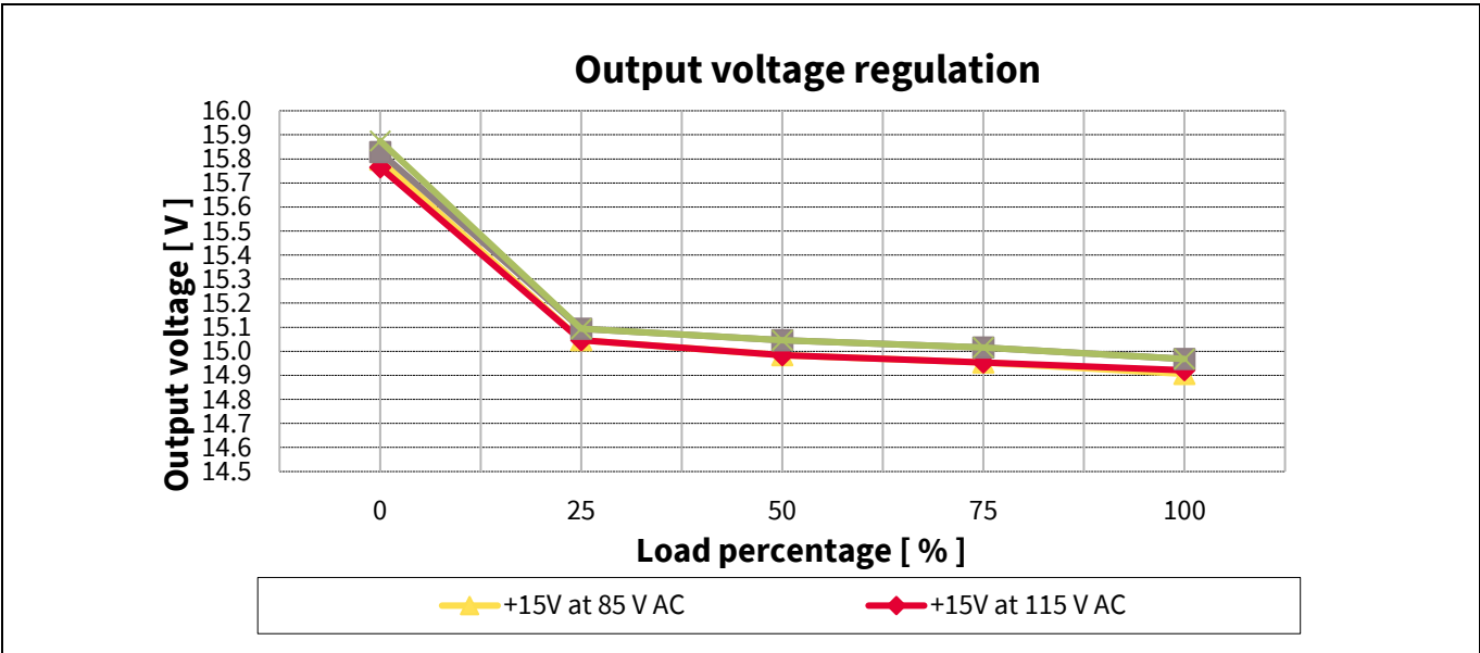
Figure 25 Output voltage regulation – design example B
