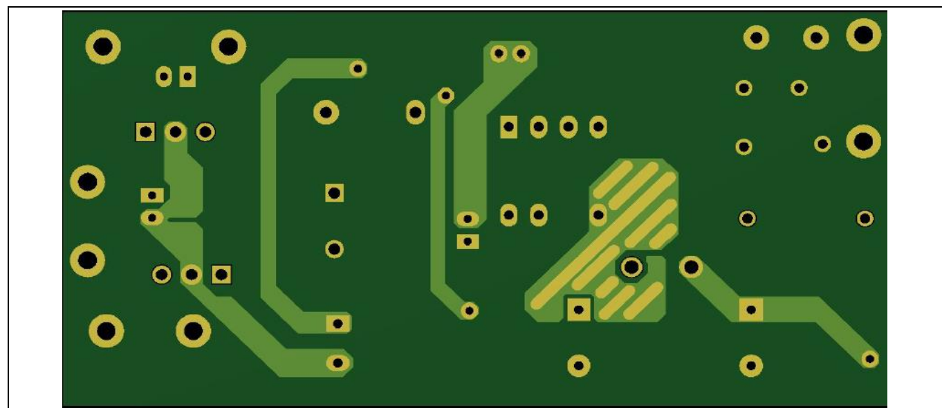
Figure 5 Bottom-side copper
