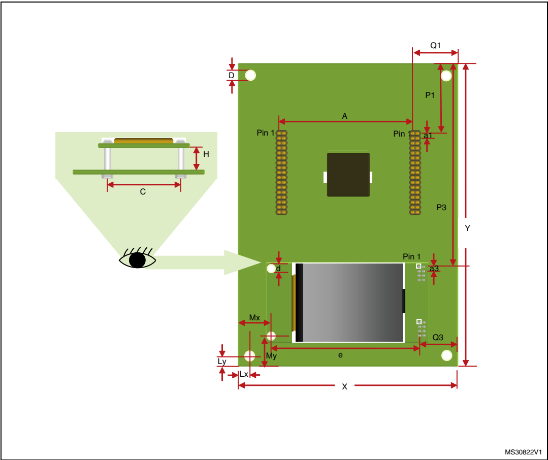
Figure 31. Mechanical dimensions
