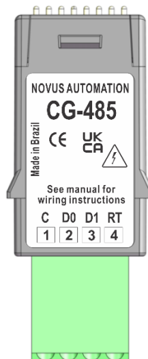
Figure 2 – Electrical connections
