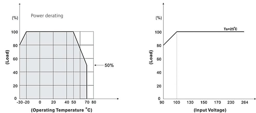
Derating graphs
