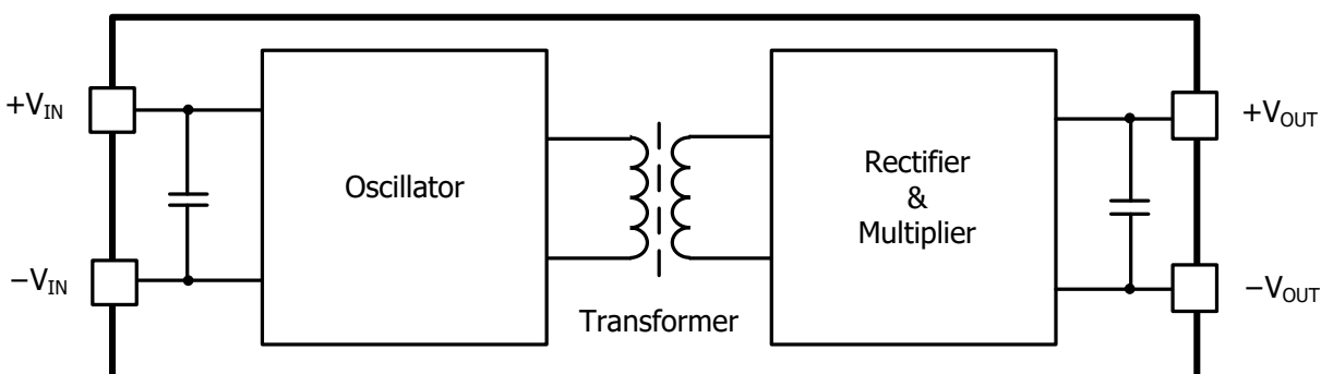
Figure 4. Block Diagram
