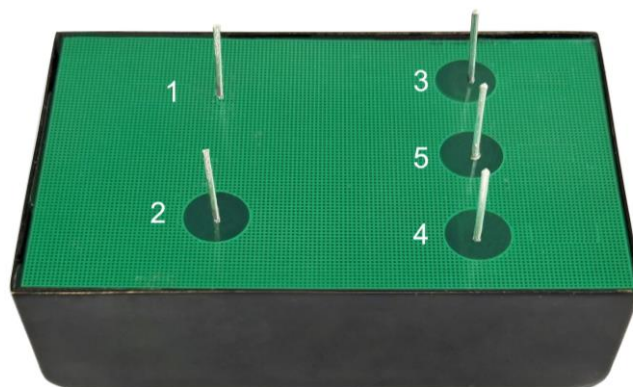
Figure 1. Physical Photos of AHVR15V4KV2R5MAP
