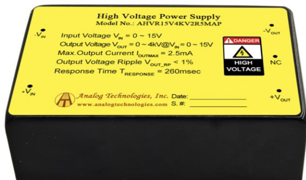
Figure 1. Physical Photos of AHVR15V4KV2R5MAP
