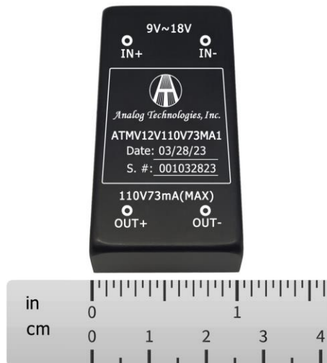
Figure 1. Top View
