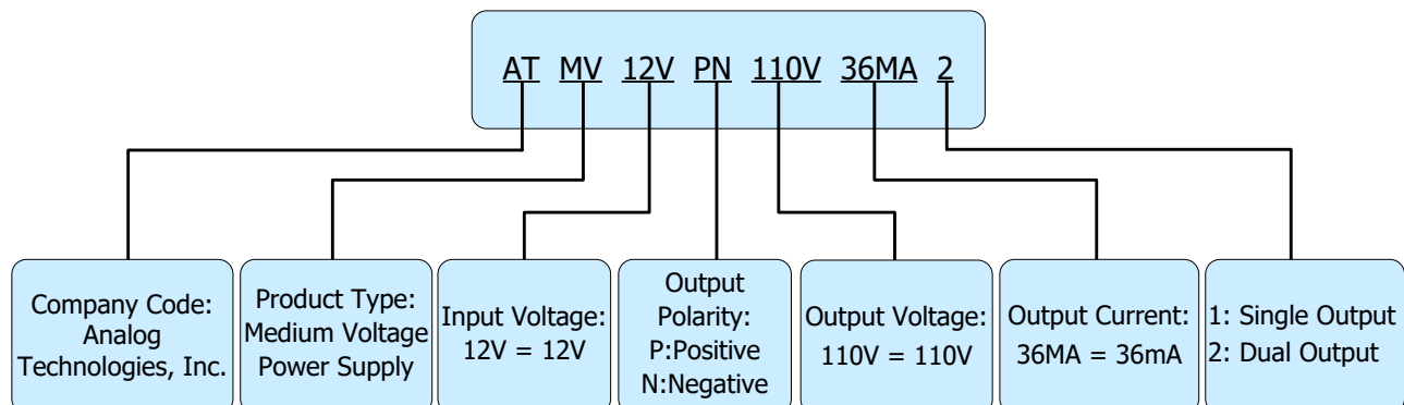
Figure 7. Naming Principle of ATMV12VPN110V36MA2
