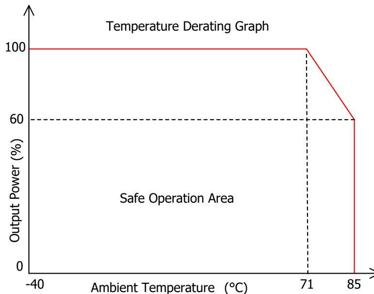
Figure 5. Derating Curve
