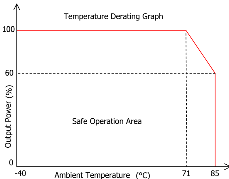
Figure 5. Derating Curve
