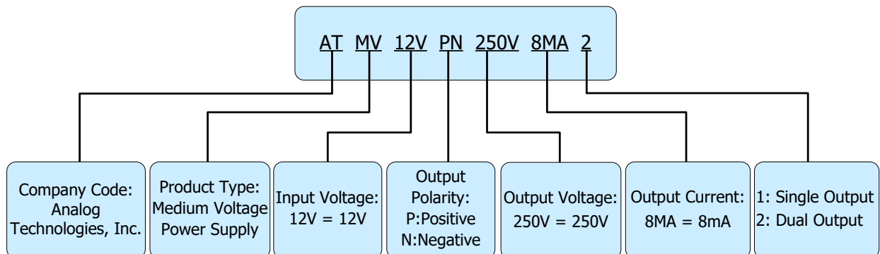
Figure 7. Naming Principle of ATMV12VPN250V8MA2
