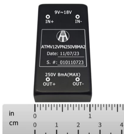
Figure 1. Top View of ATMV12VPN250V8MA2
