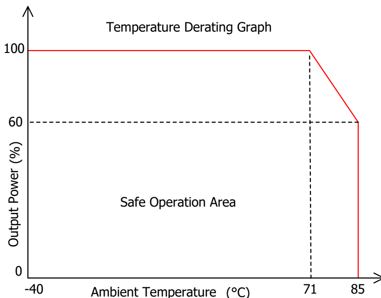
Figure 5. Derating Curve
